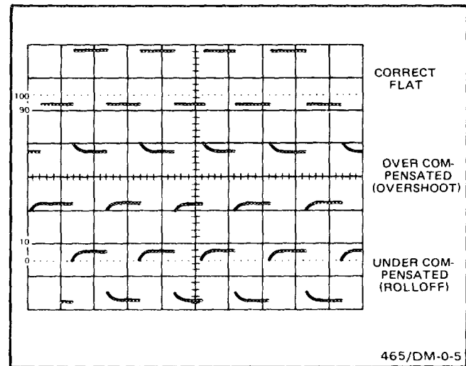
Fig. 11. Probe compensation.
