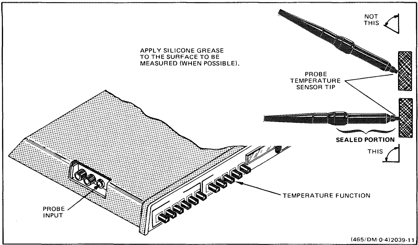
Fig. 10. Temperature.
