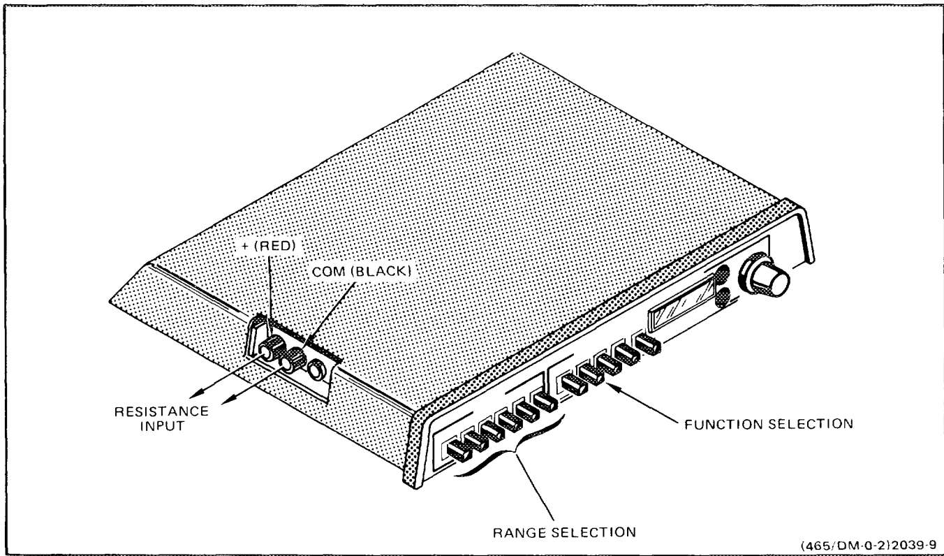
Fig. 8. Resistance.
