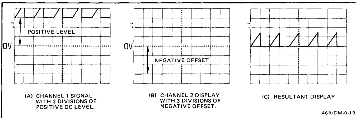
Fig. 16. Algebraic addition.
