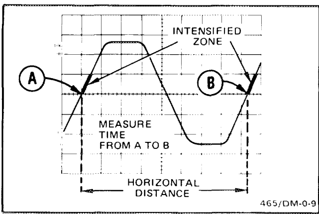
Fig. 26. Time duration.
